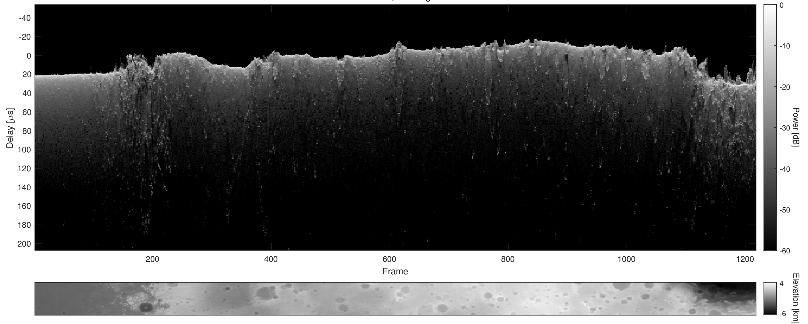
Orbit 11399, Cluttergram
