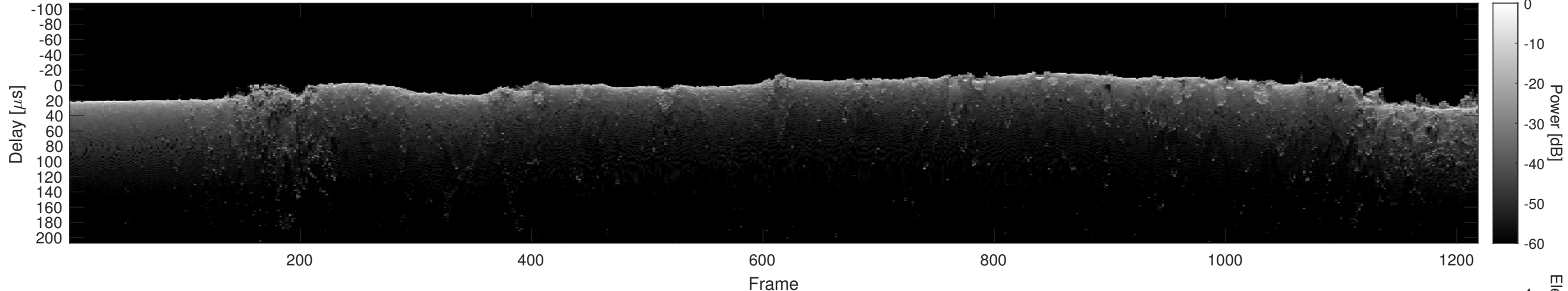
Orbit 11399, Cluttergram
