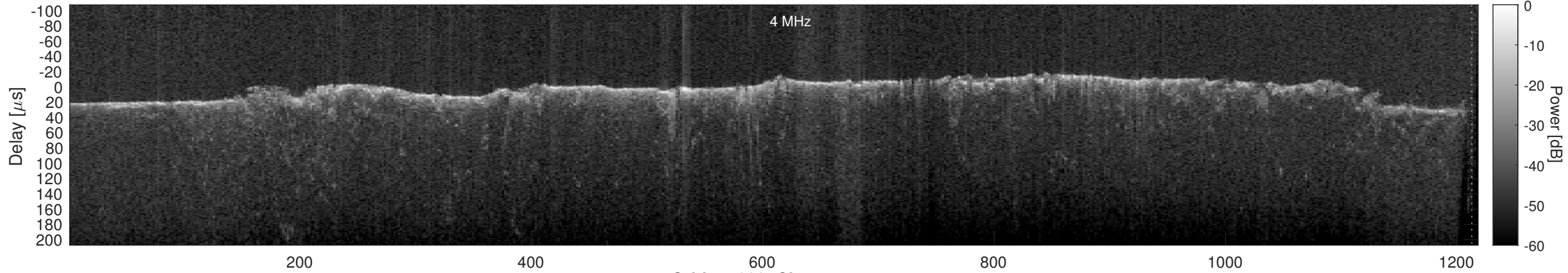
Orbit 11399, Cluttergram
