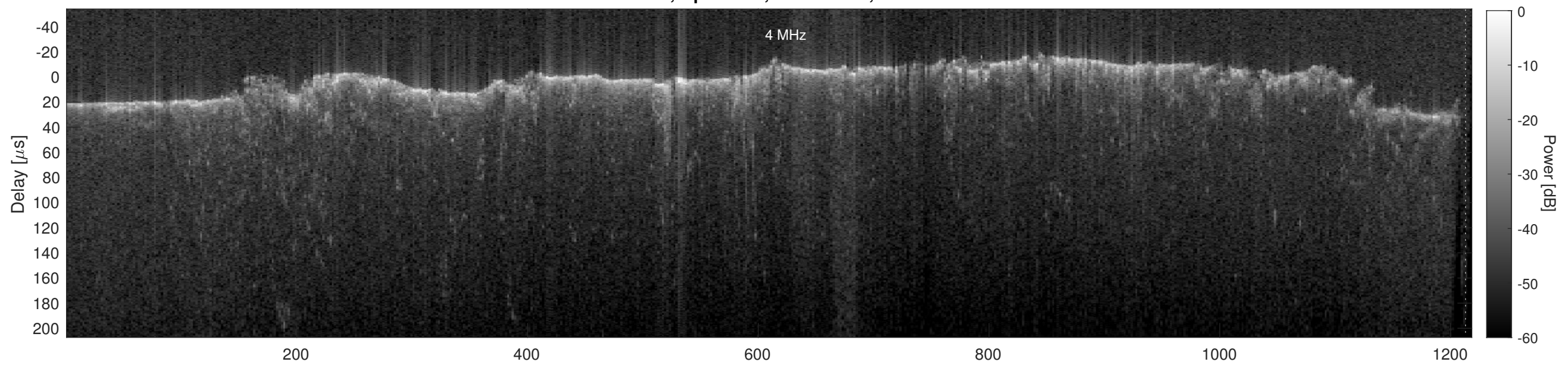
Orbit 11399, Cluttergram
