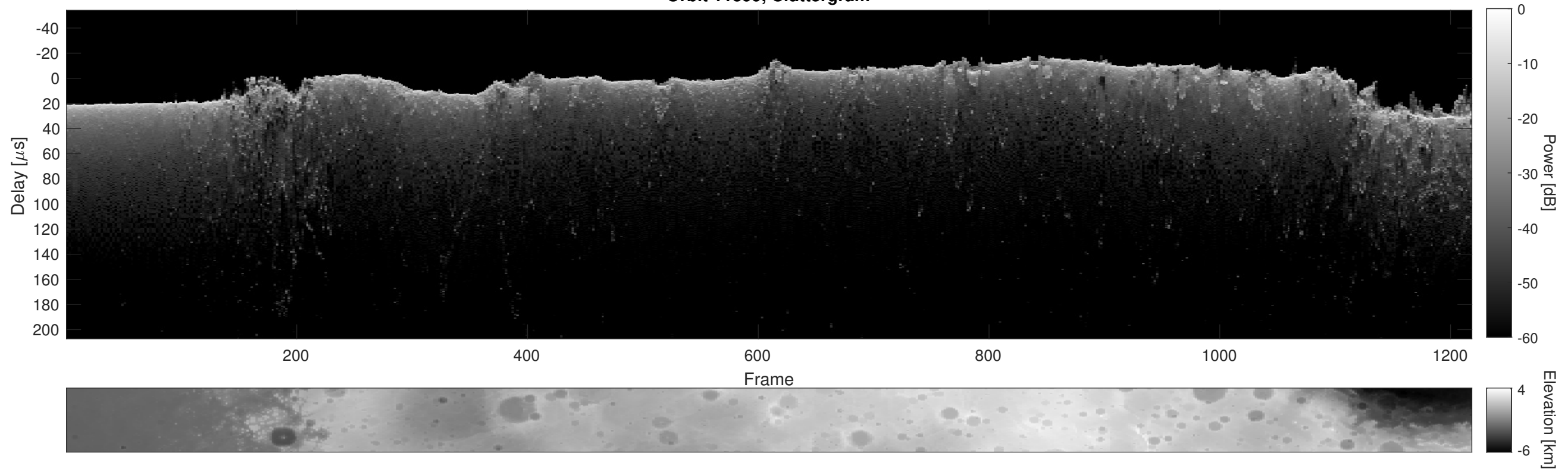
Orbit 11399, Cluttergram
