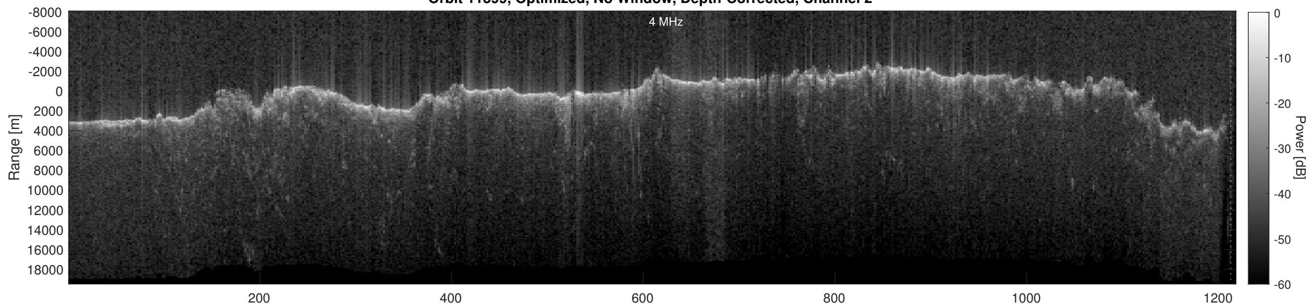
Orbit 11399, Depth-Corrected Cluttergram
