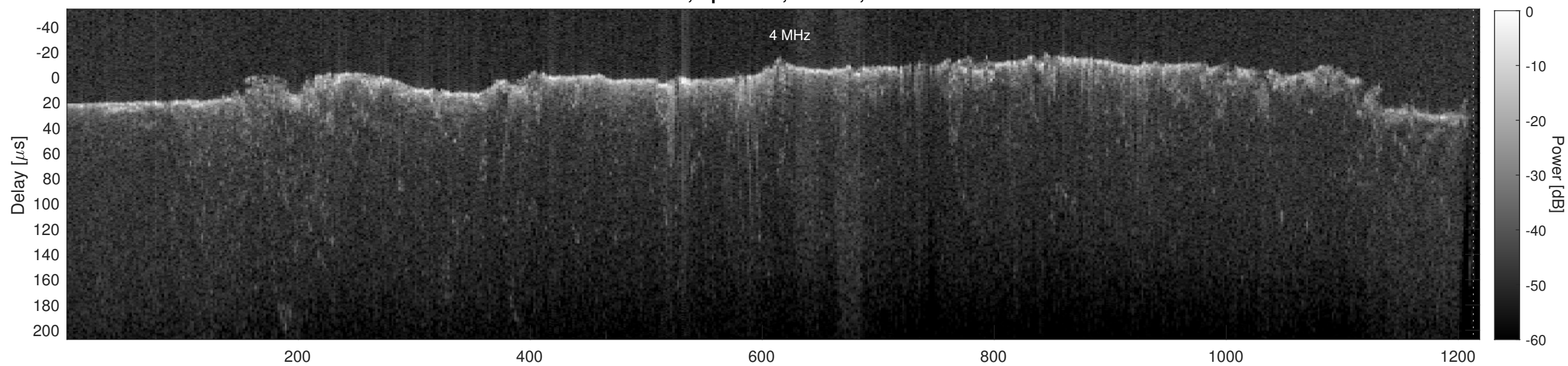
Orbit 11399, Cluttergram
