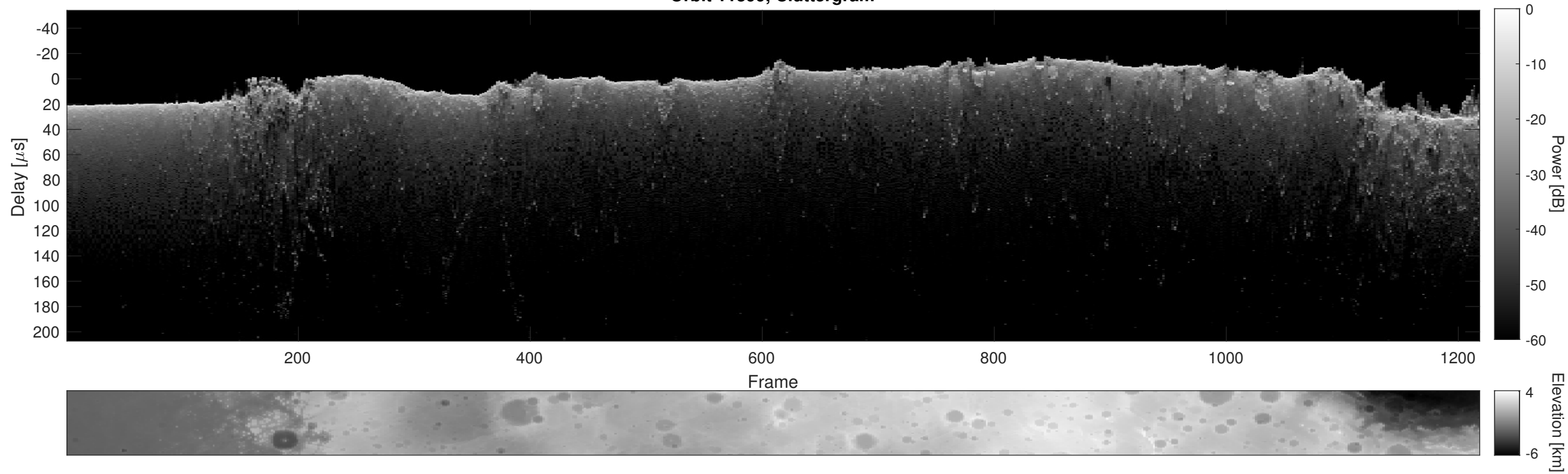
Orbit 11399, Cluttergram
