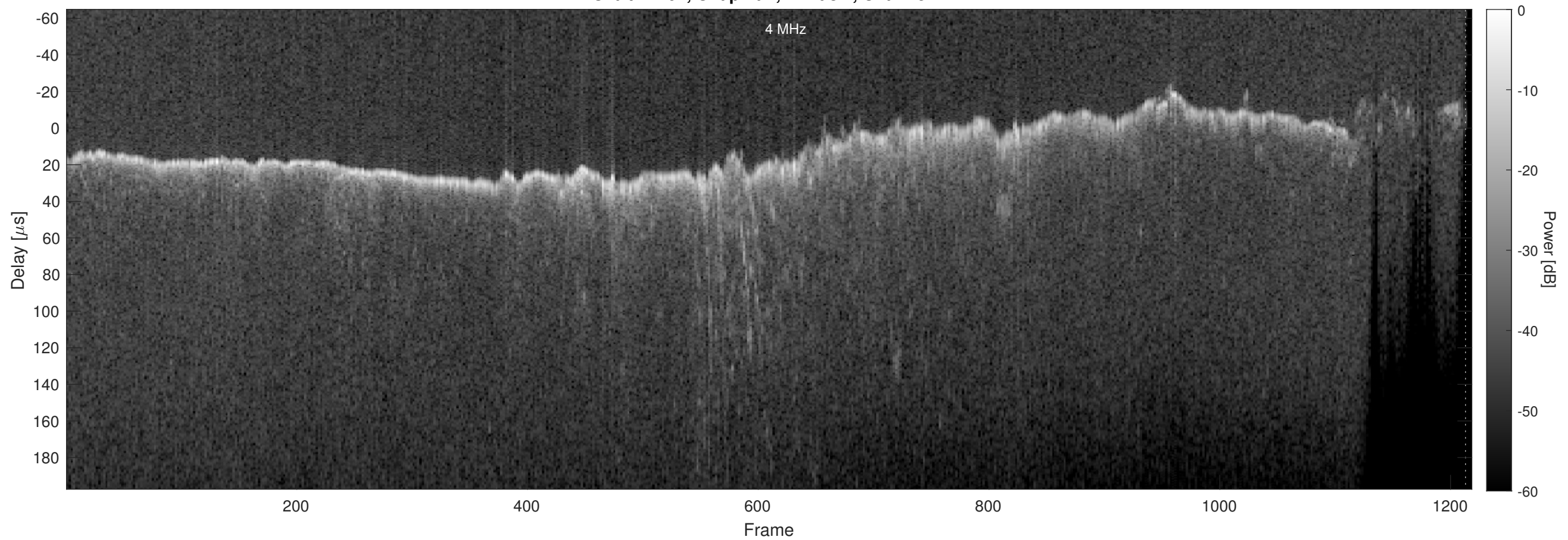
Orbit 11402, Chapman, Window, Channel 2
