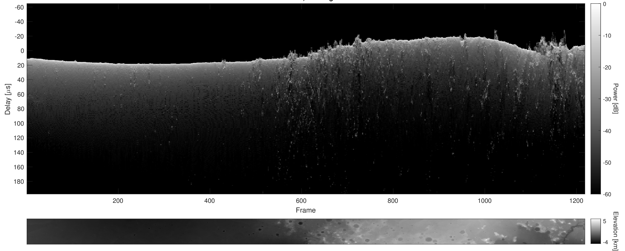
Orbit 11402, Cluttergram
