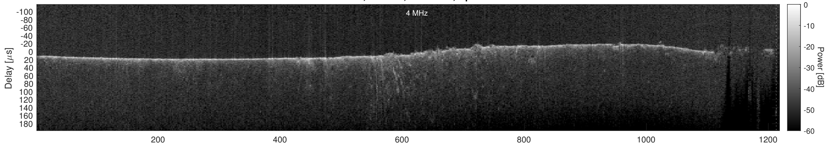
Orbit 11402, Cluttergram
