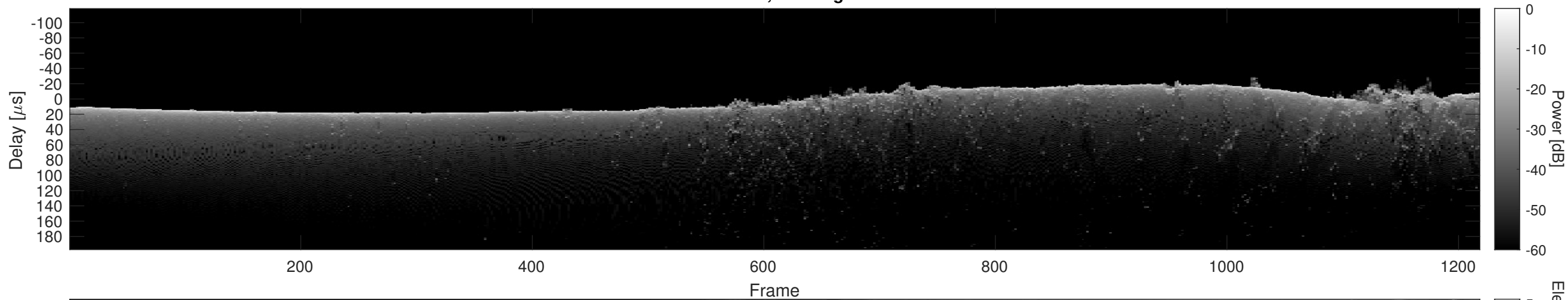
Orbit 11402, Cluttergram
