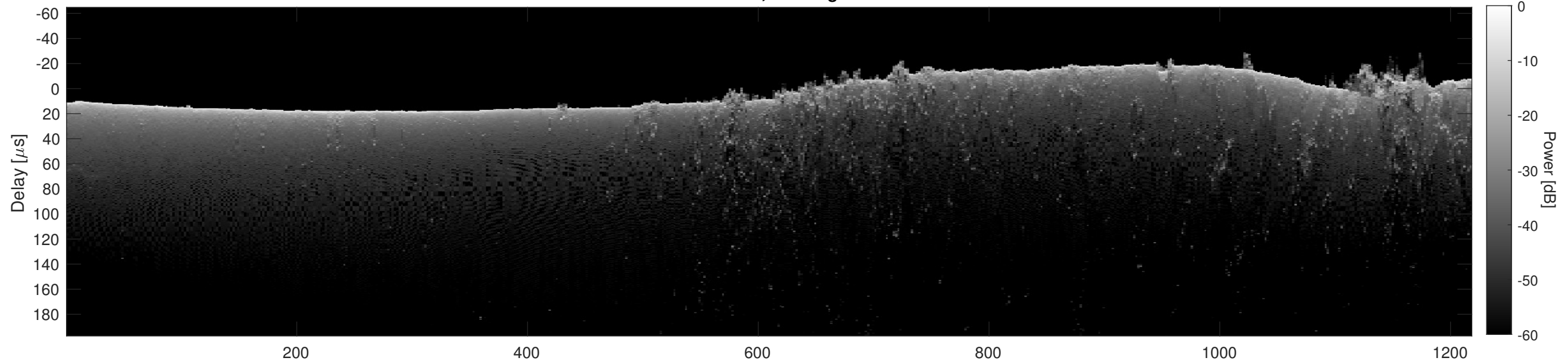
Orbit 11402, Cluttergram
