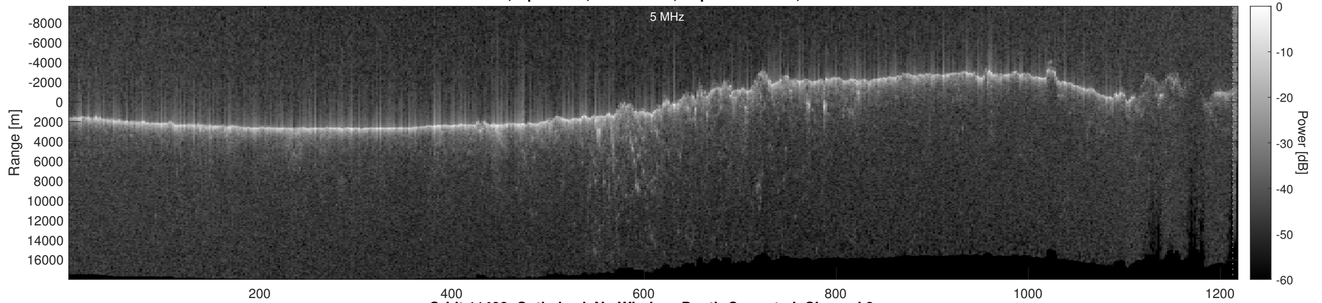
Orbit 11402, Optimized, No Window, Depth-Corrected, Channel 2
