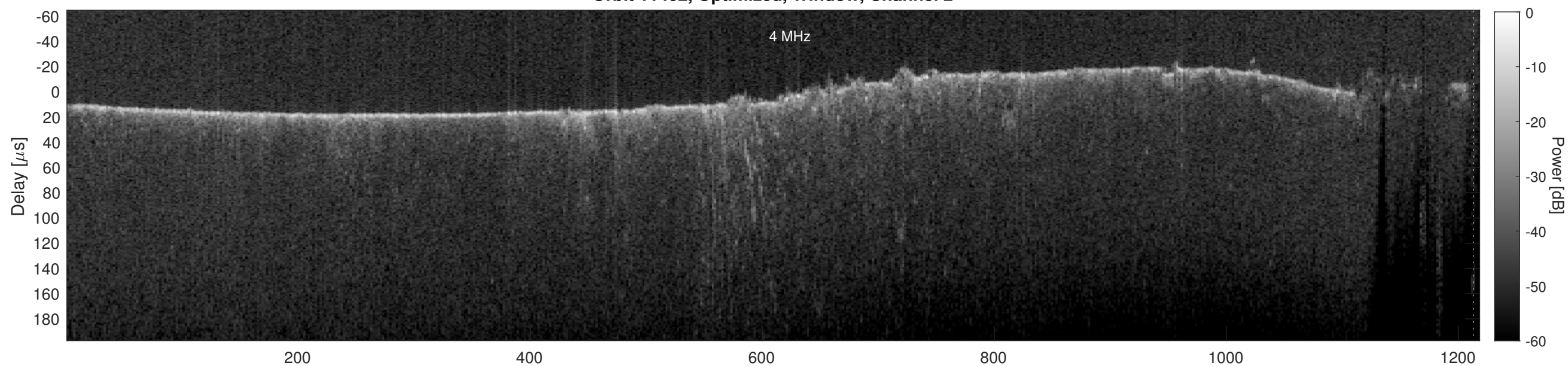
Orbit 11402, Cluttergram
