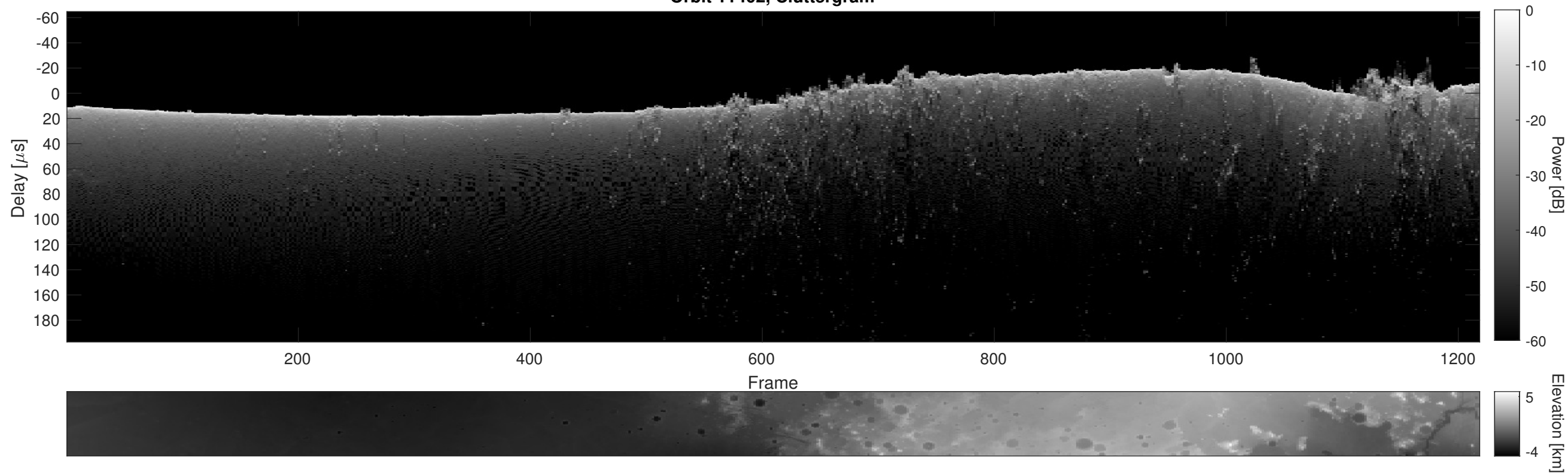
Orbit 11402, Cluttergram
