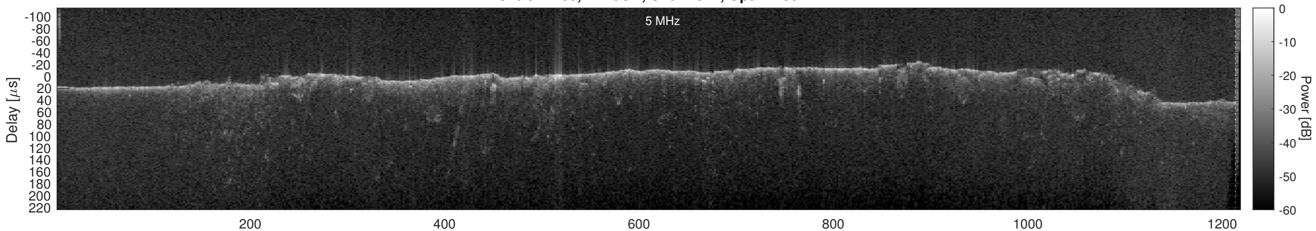
Orbit 11406, Cluttergram
