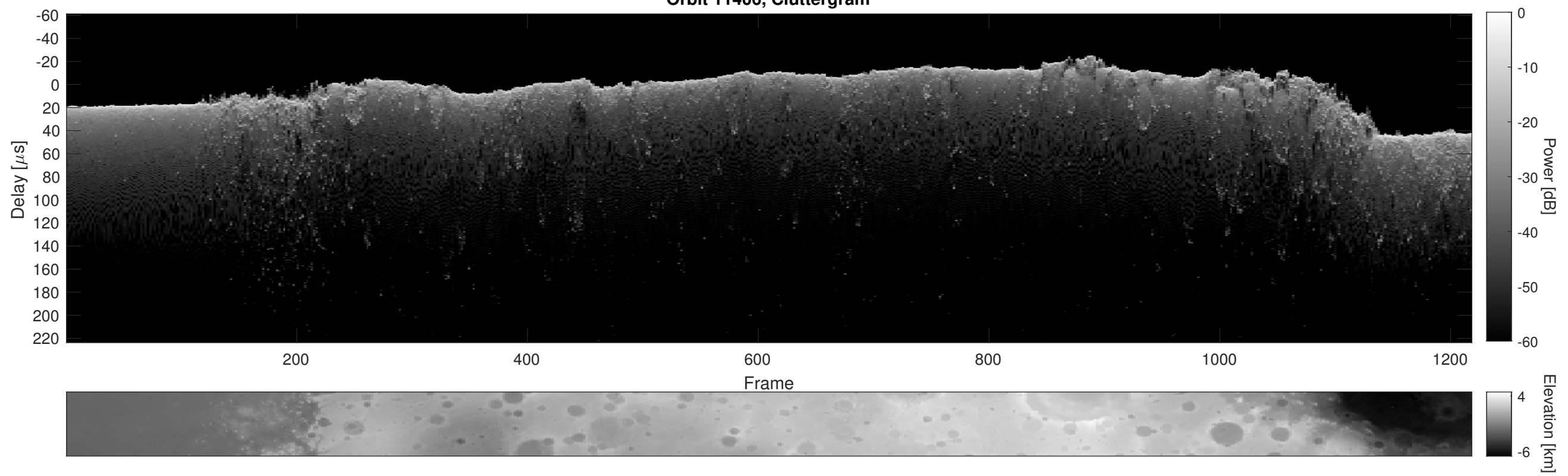
Orbit 11406, Cluttergram
