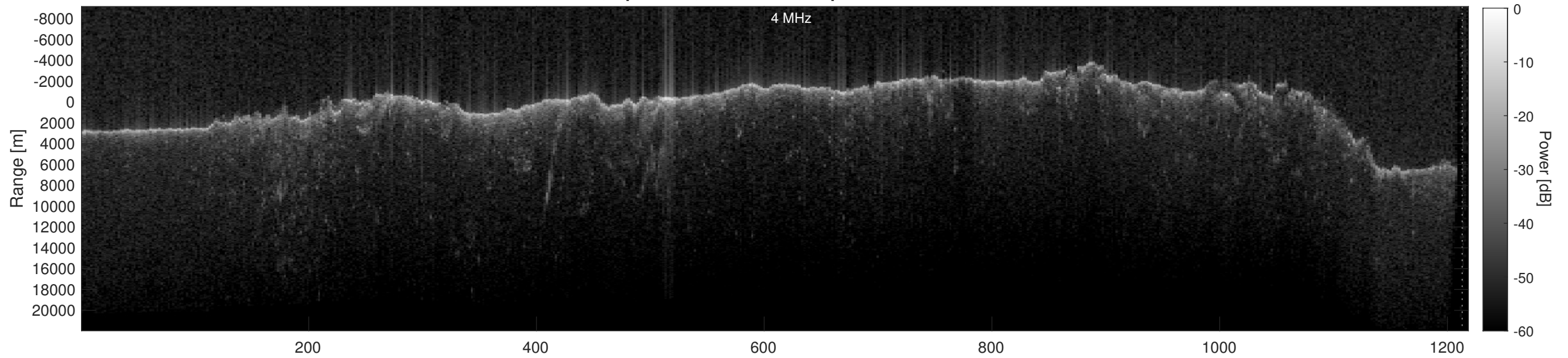
Orbit 11406, Depth-Corrected Cluttergram
