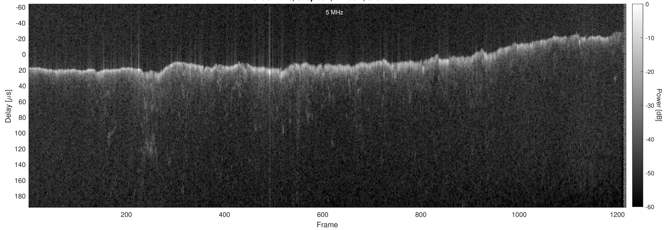
Orbit 11410, Chapman, Window, Channel 2
