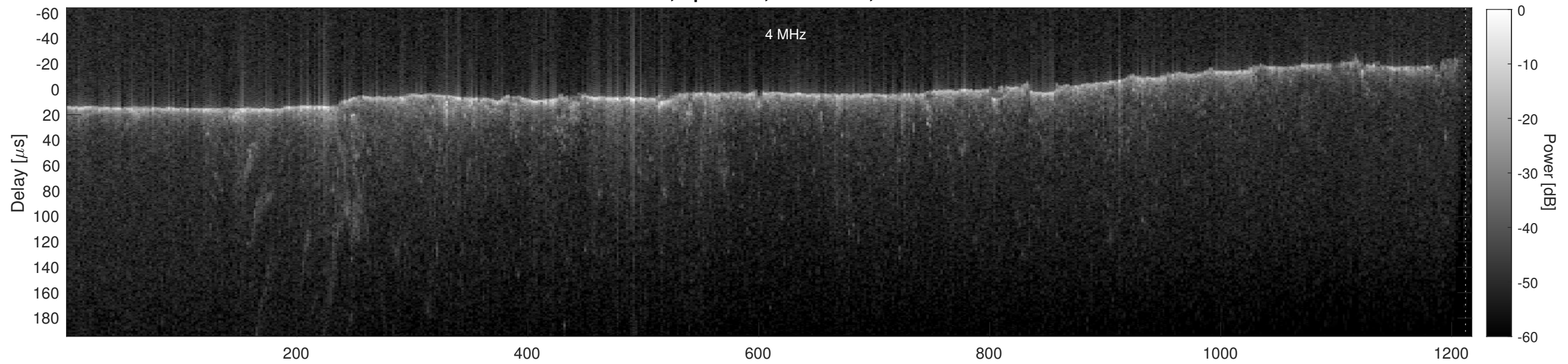
Orbit 11410, Cluttergram
