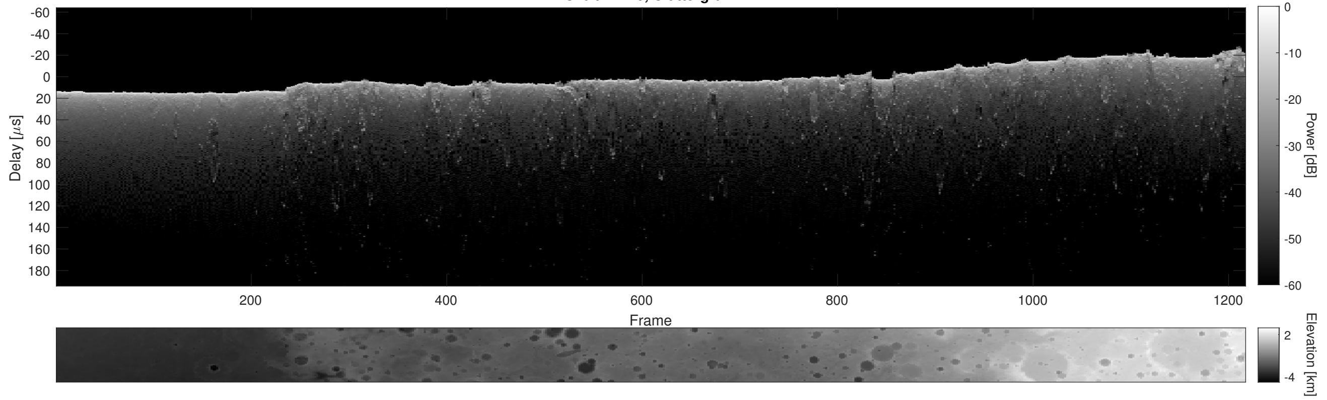
Orbit 11410, Cluttergram
