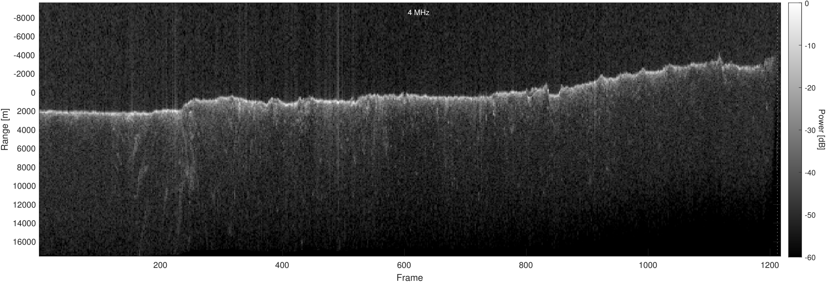
Orbit 11410, Optimized, Window, Depth-Corrected, Channel 2
