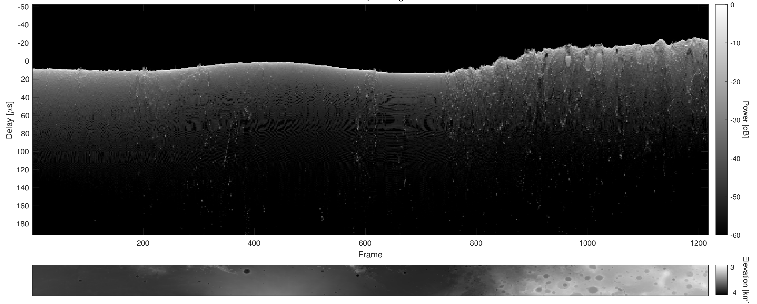
Orbit 11412, Cluttergram
