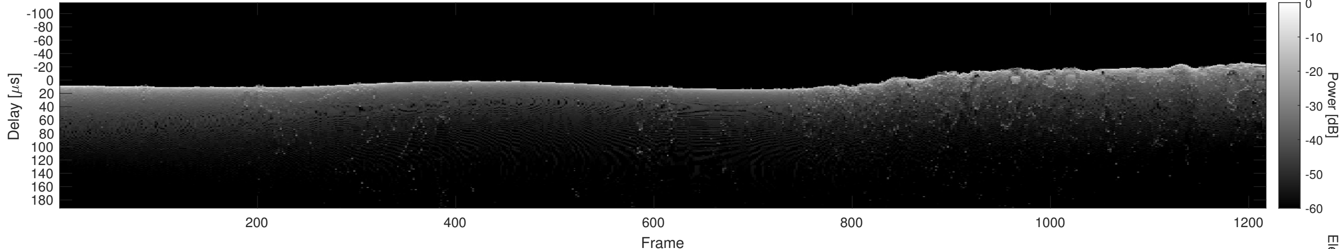
Orbit 11412, Cluttergram
