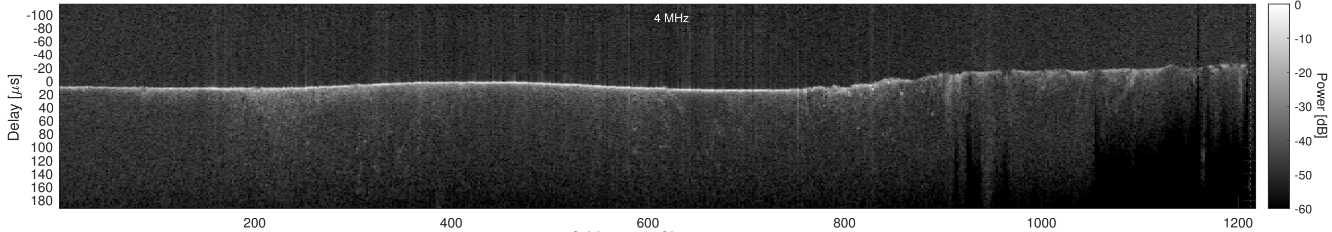
Orbit 11412, Cluttergram
