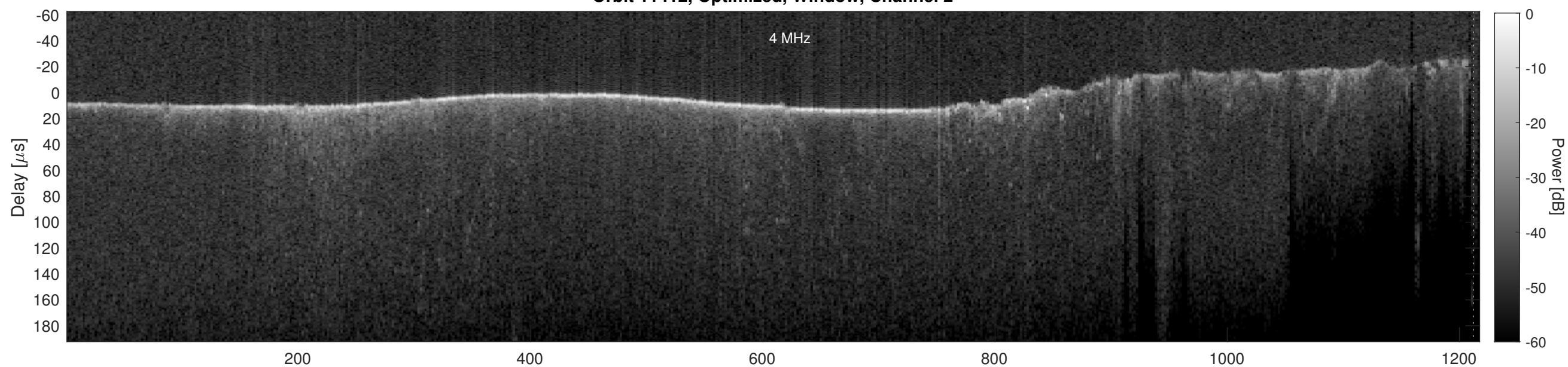
Orbit 11412, Cluttergram
