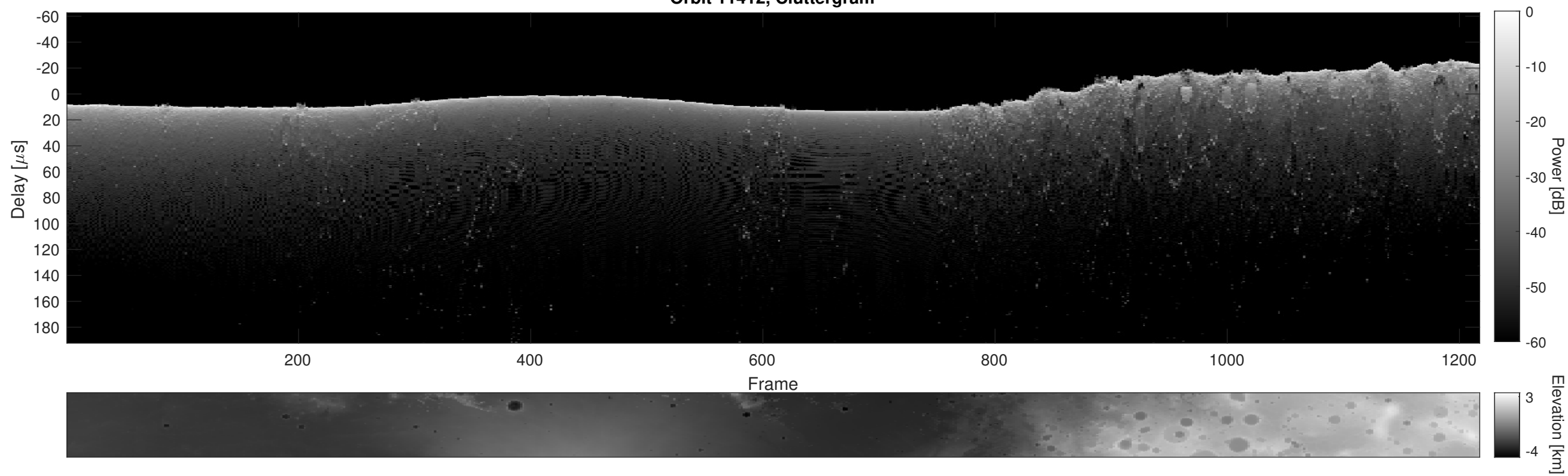
Orbit 11412, Cluttergram
