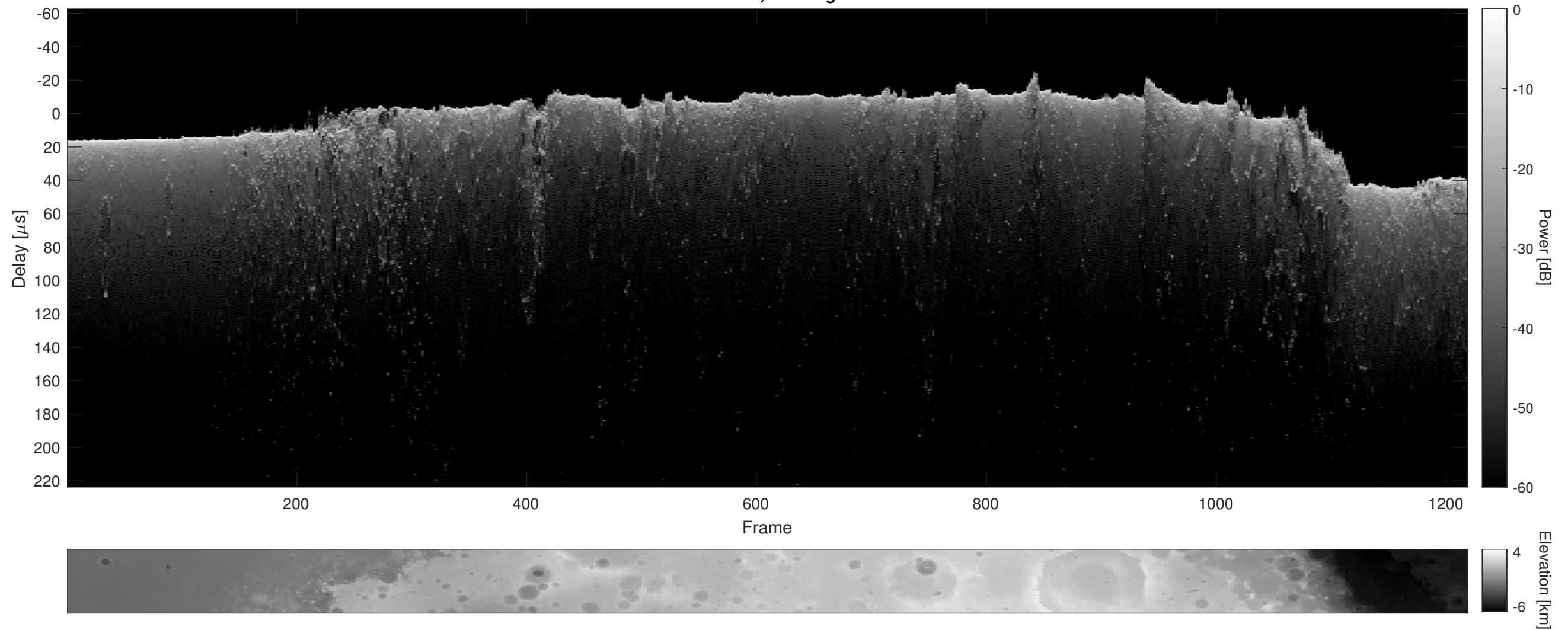
Orbit 11413, Cluttergram
