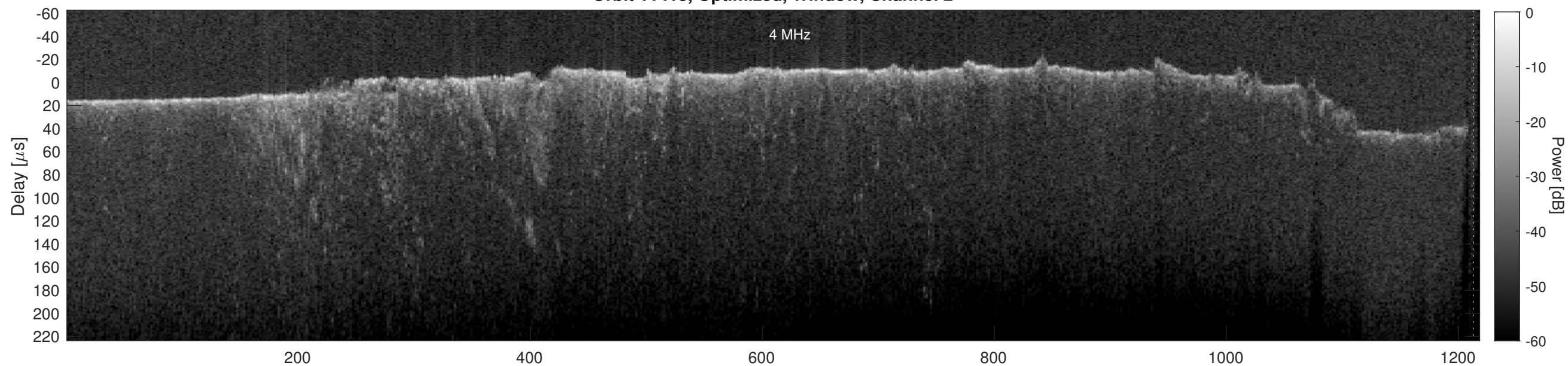
Orbit 11413, Cluttergram
