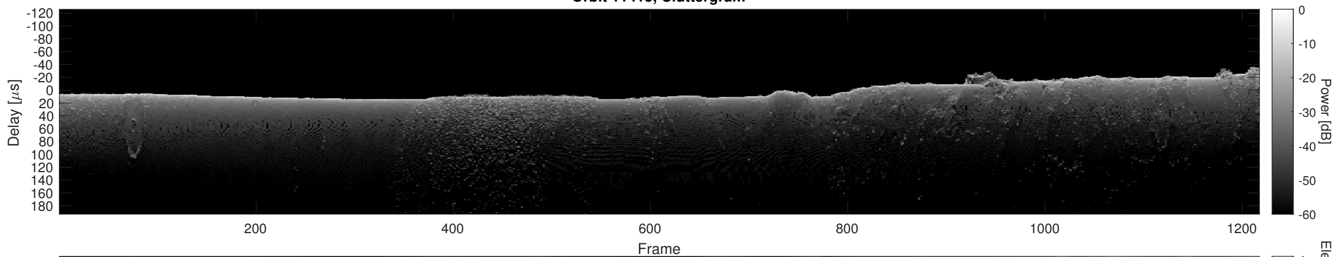
Orbit 11415, Cluttergram
