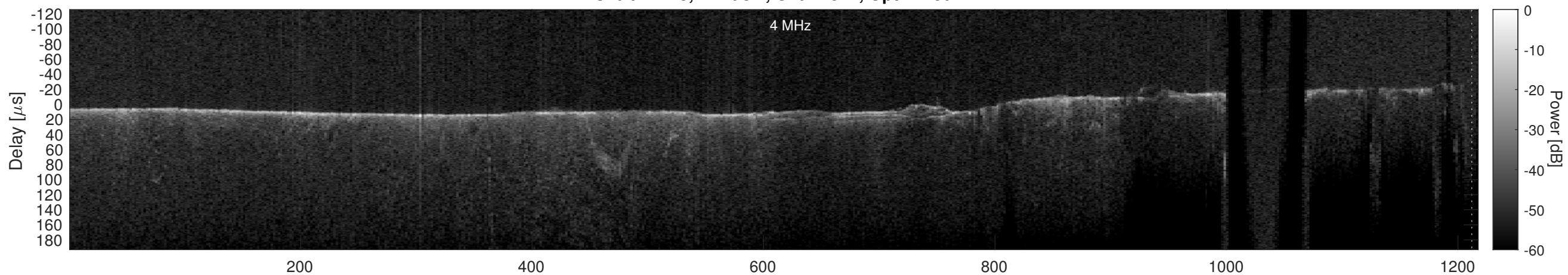
Orbit 11415, Cluttergram
