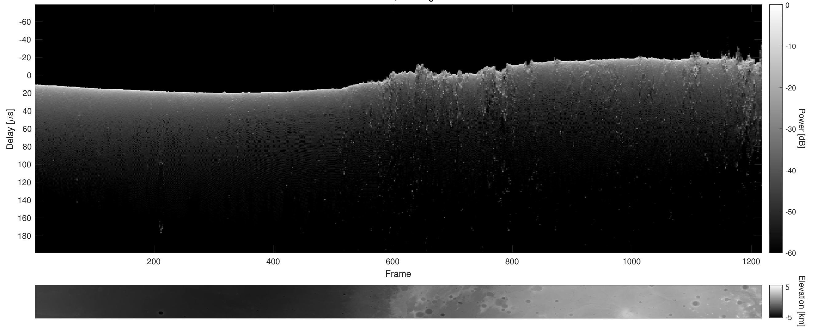
Orbit 11416, Cluttergram
