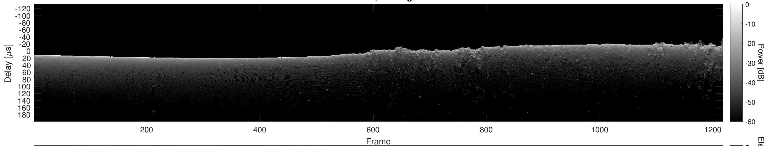
Orbit 11416, Cluttergram
