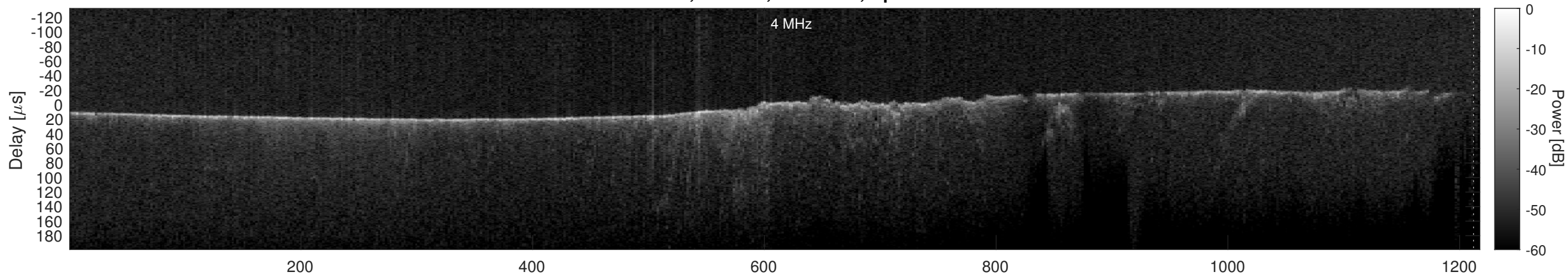
Orbit 11416, Cluttergram
