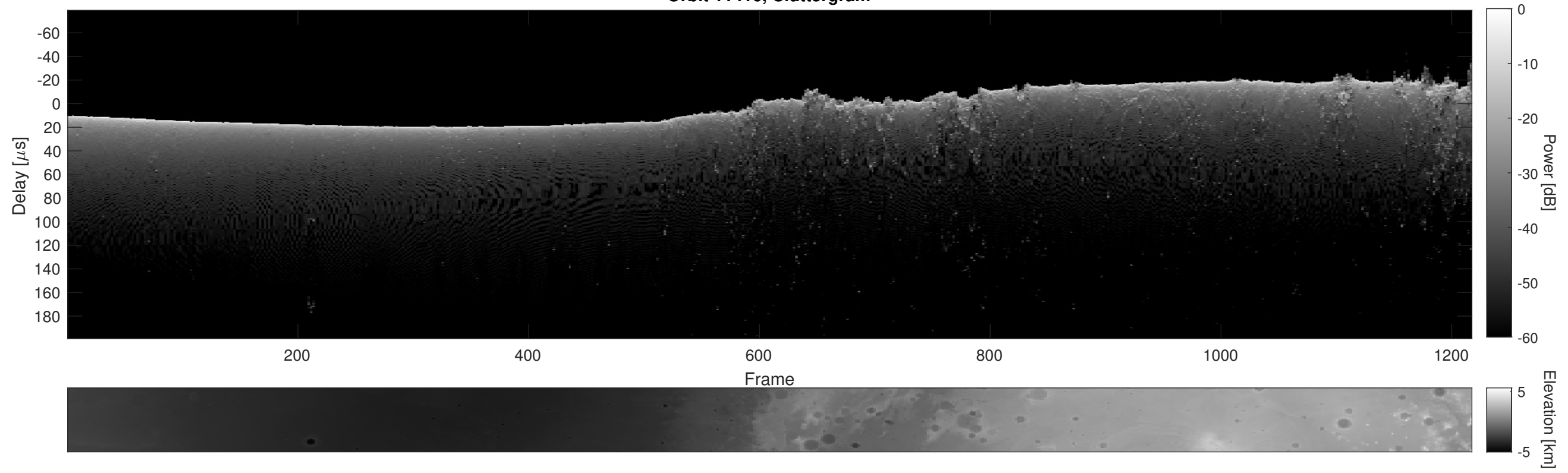
Orbit 11416, Cluttergram
