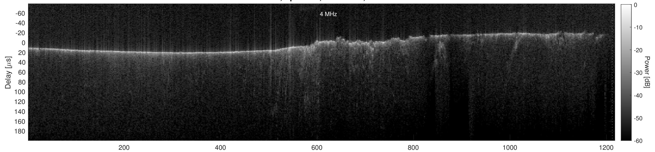
Orbit 11416, Cluttergram
