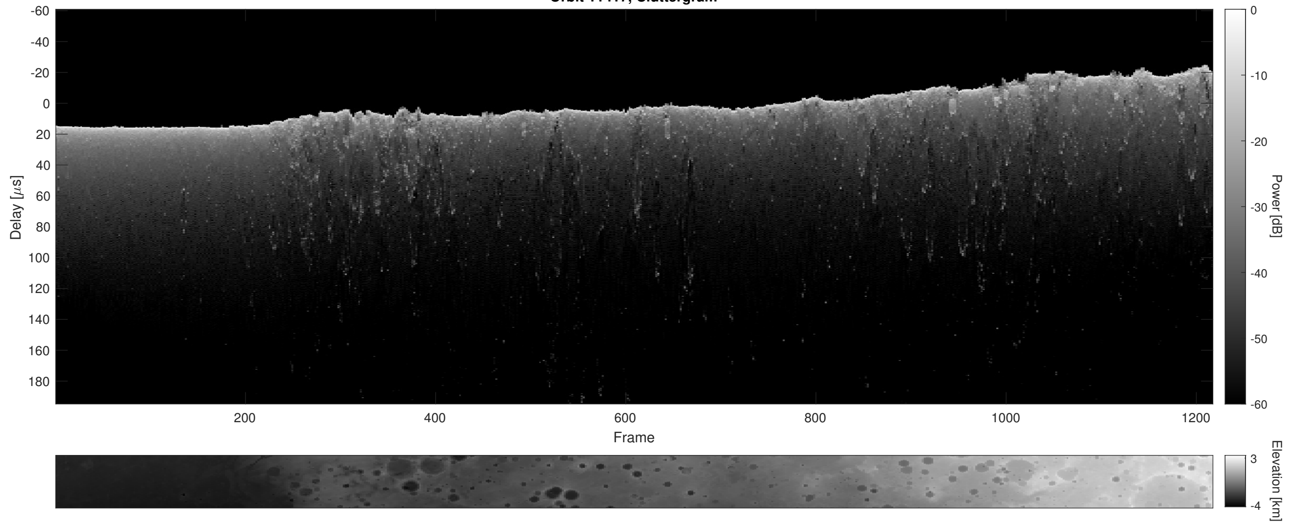
Orbit 11417, Cluttergram
