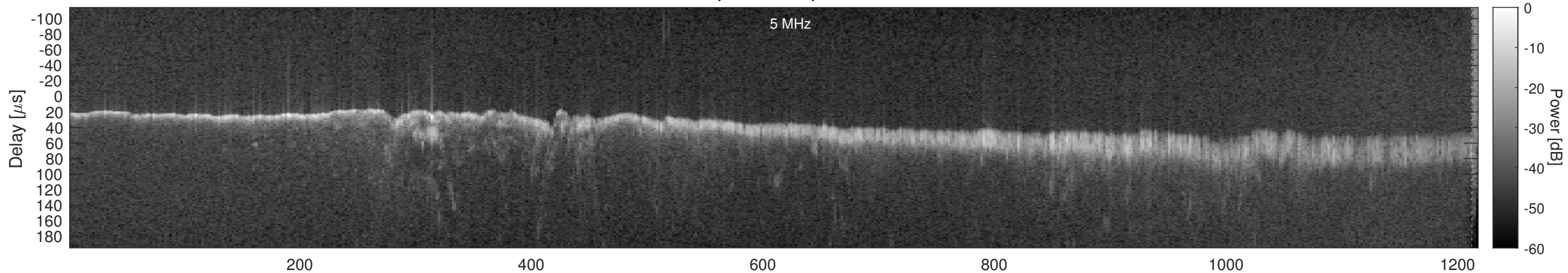
Orbit 11417, Window, Channel 1, Chapman
