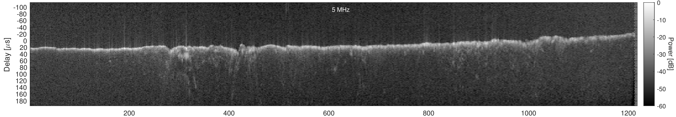
Orbit 11417, Window, Channel 1, Optimized
