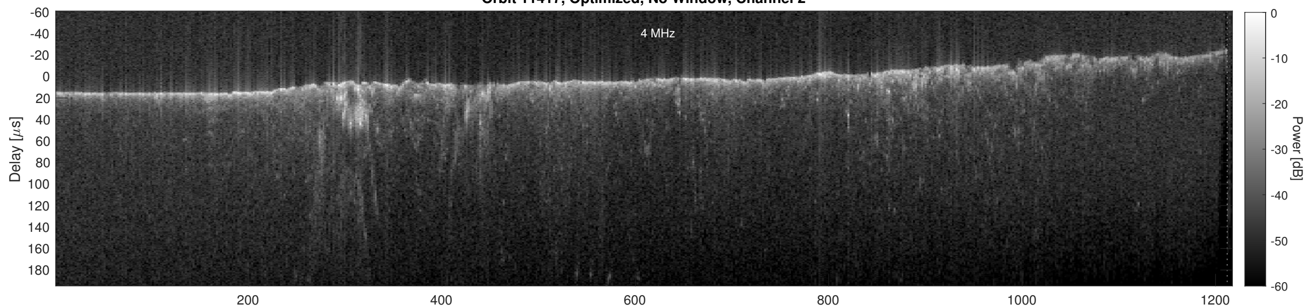
Orbit 11417, Cluttergram
