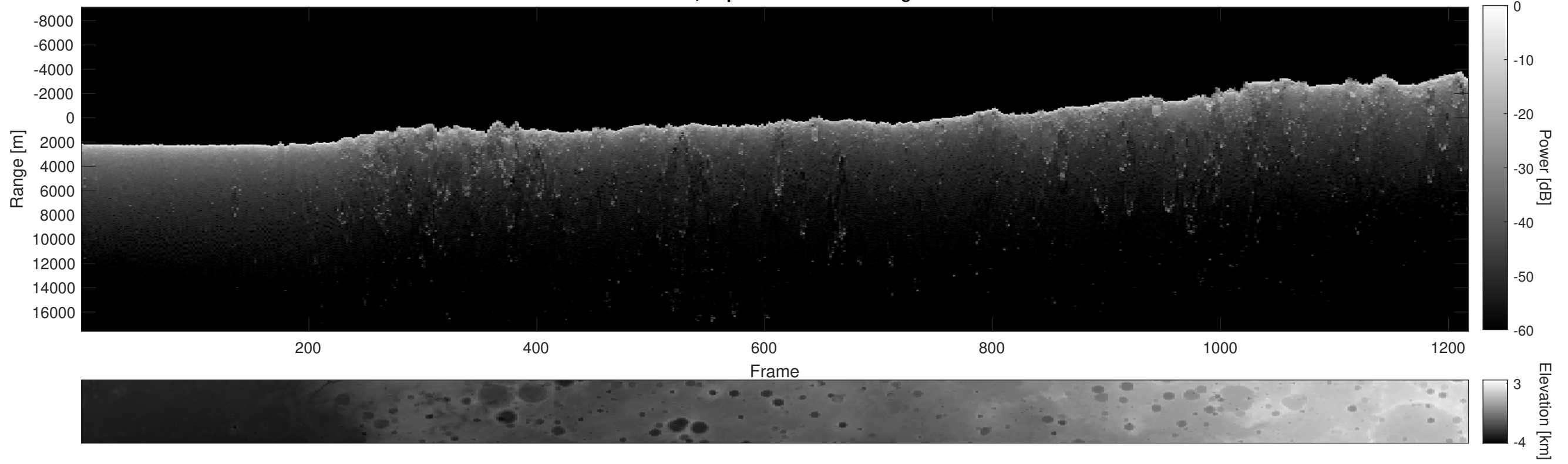
Orbit 11417, Depth-Corrected Cluttergram
