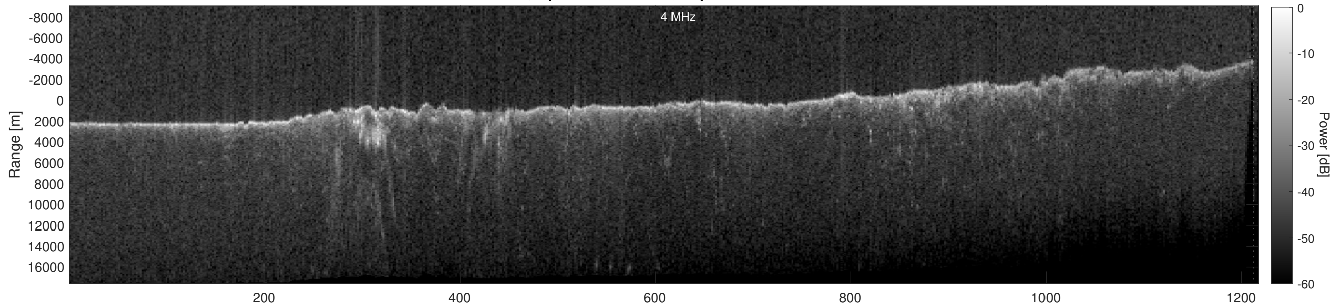
Orbit 11417, Depth-Corrected Cluttergram
