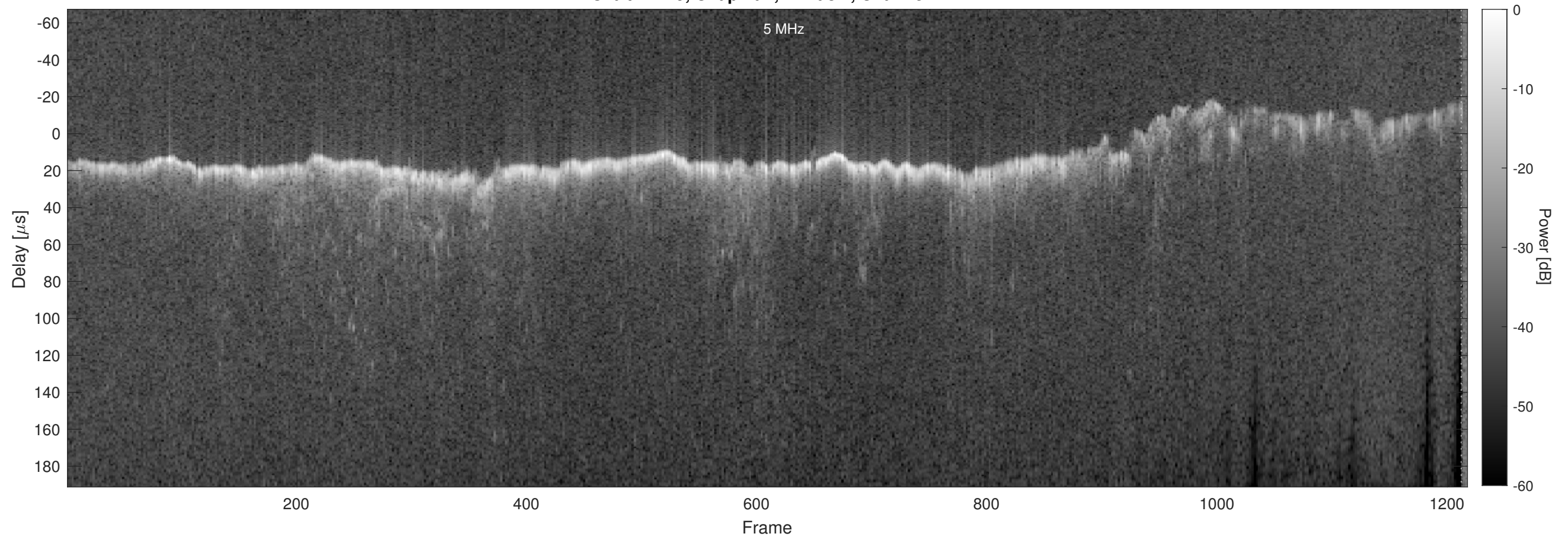
Orbit 11419, Chapman, Window, Channel 2
