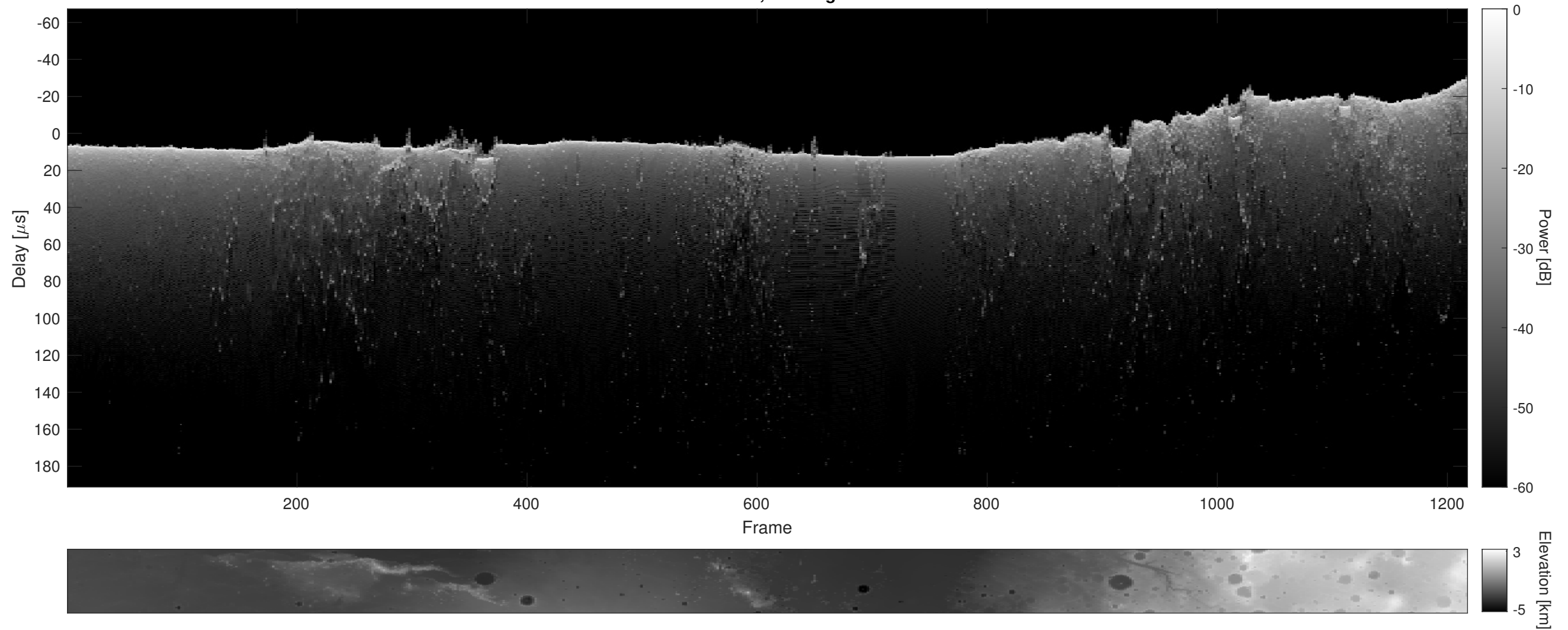
Orbit 11419, Cluttergram
