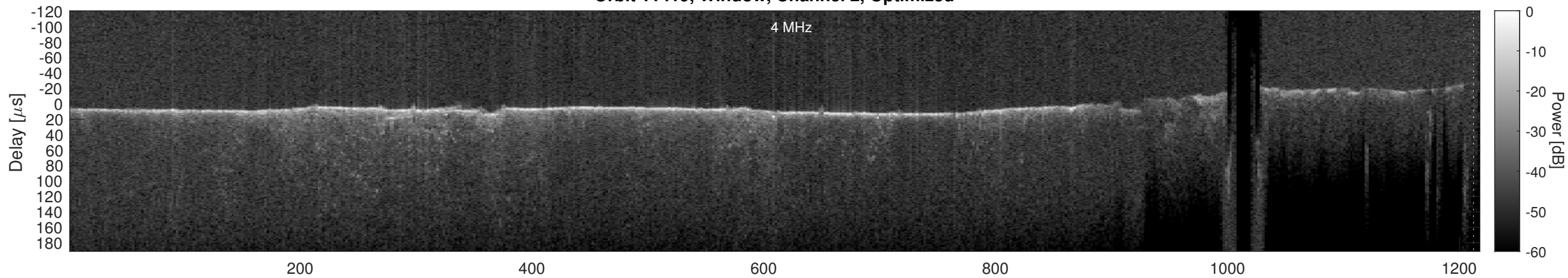
Orbit 11419, Cluttergram
