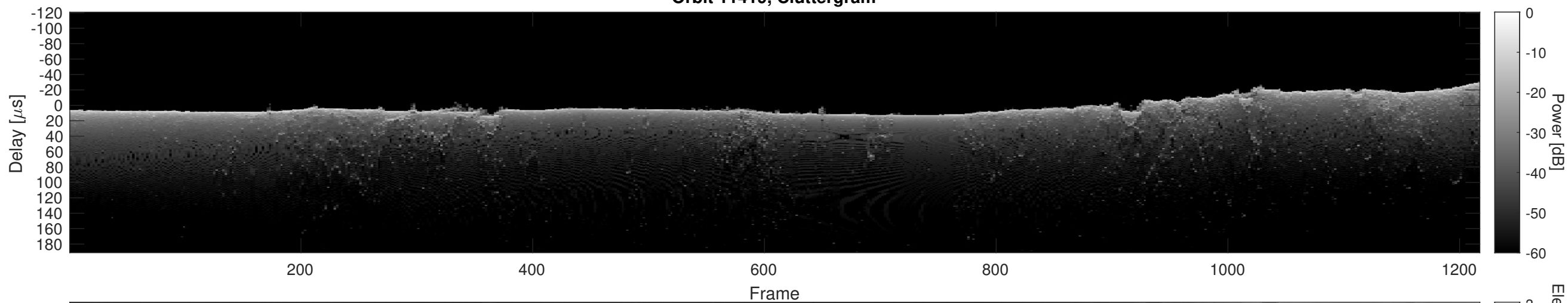
Orbit 11419, Cluttergram
