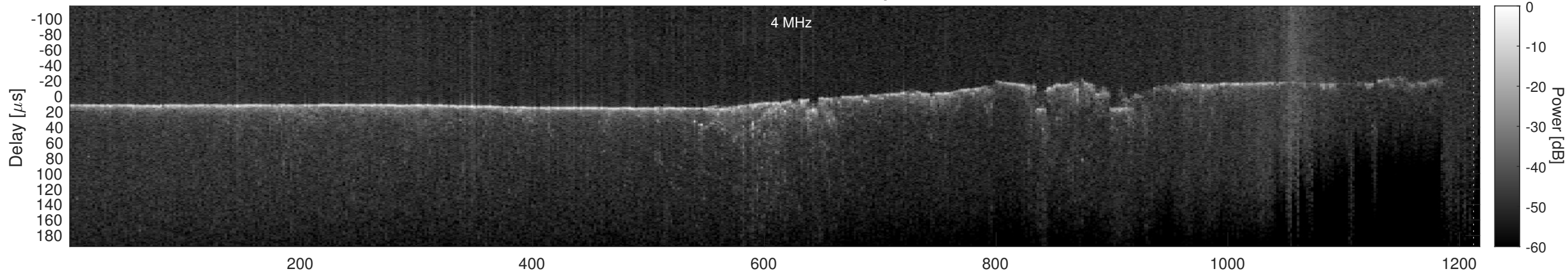
Orbit 11421, Cluttergram
