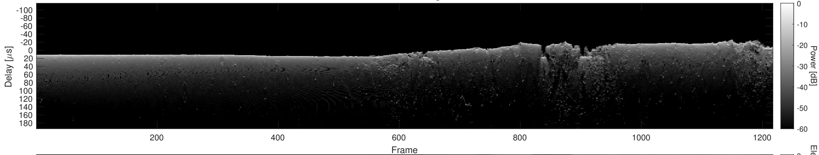
Orbit 11421, Cluttergram
