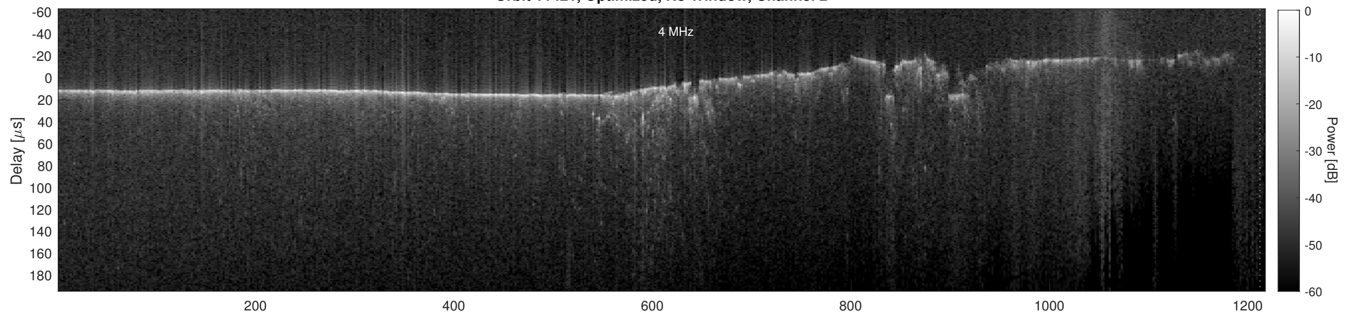
Orbit 11421, Cluttergram
