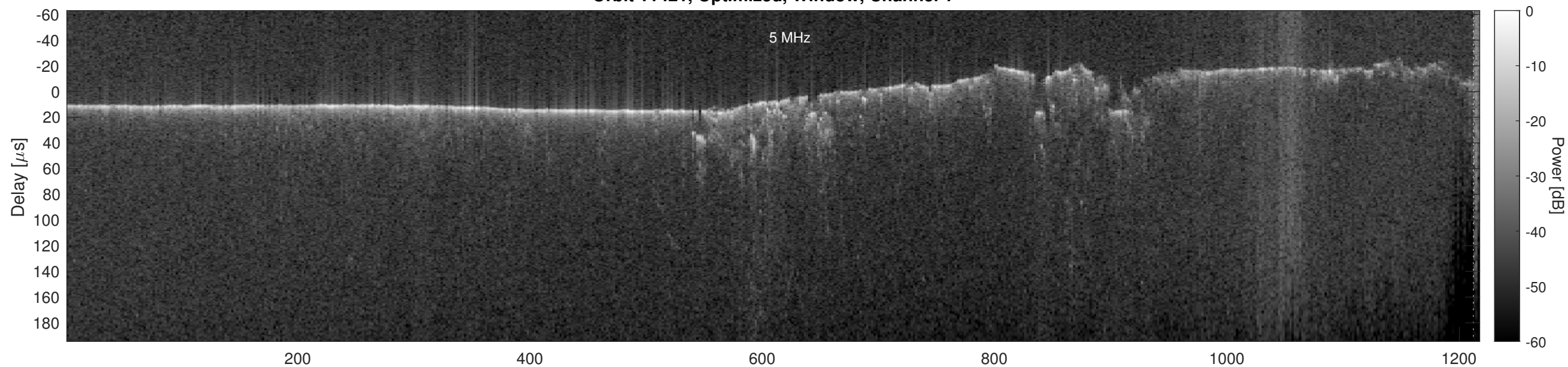
Orbit 11421, Optimized, Window, Channel 2
