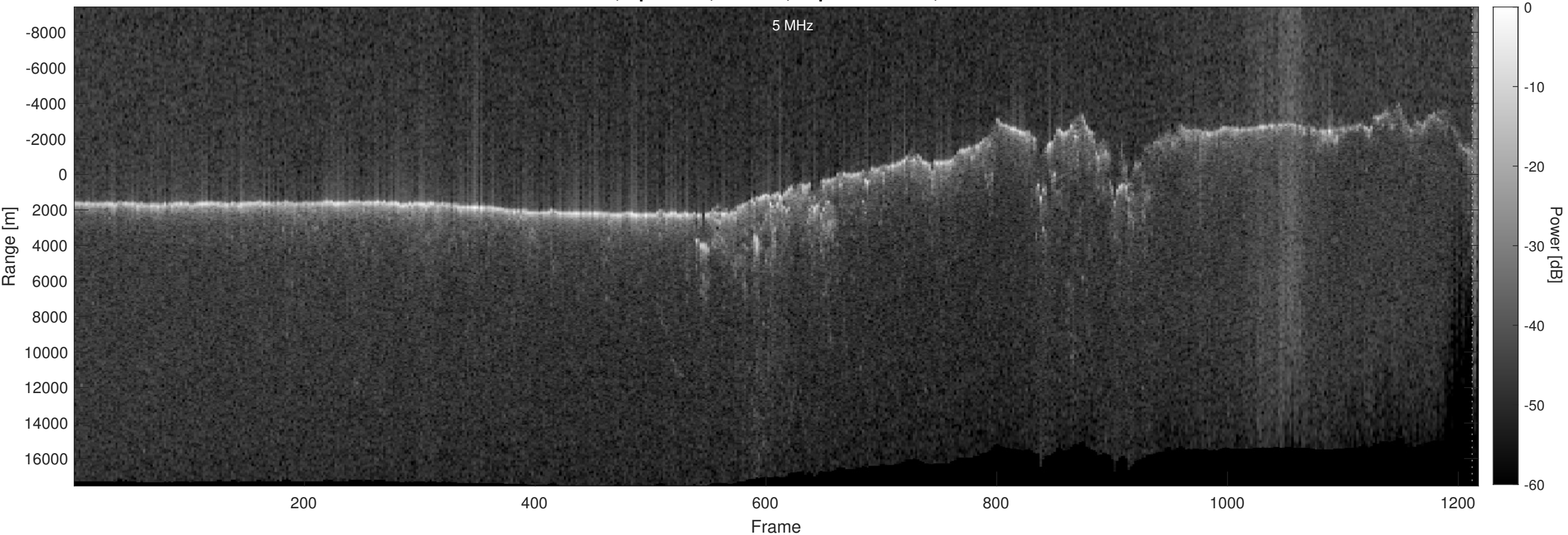
Orbit 11421, Optimized, Window, Depth-Corrected, Channel 2
