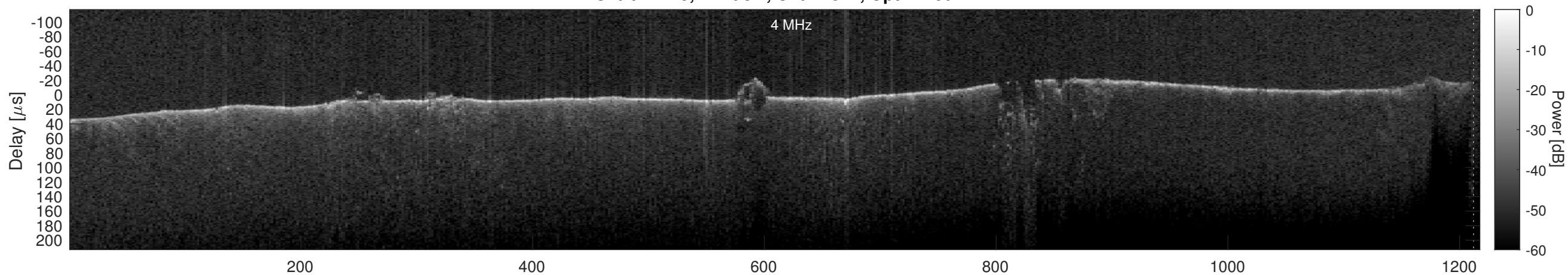
Orbit 11425, Cluttergram
