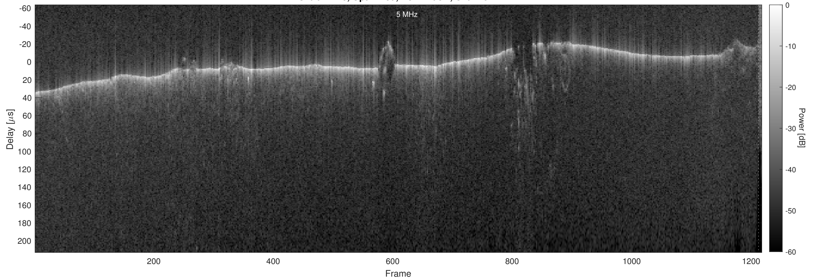
Orbit 11425, Optimized, No Window, Channel 2
