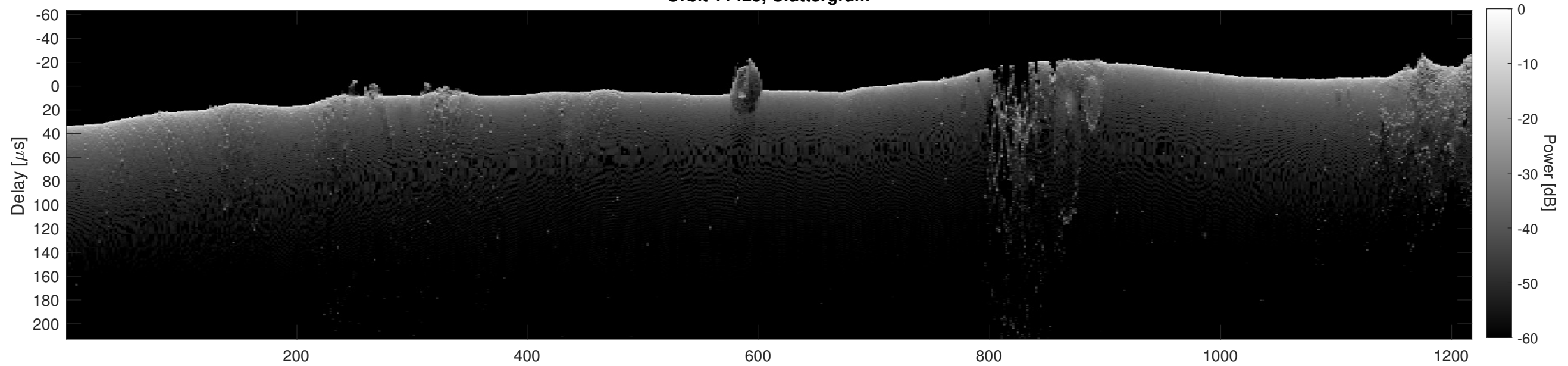
Orbit 11425, Cluttergram
