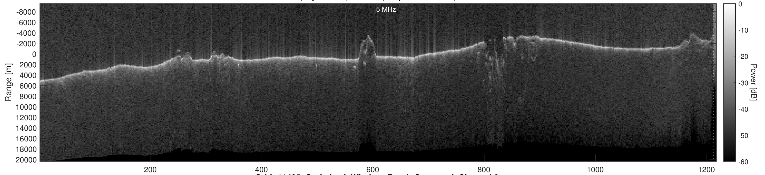
Orbit 11425, Optimized, Window, Depth-Corrected, Channel 2
