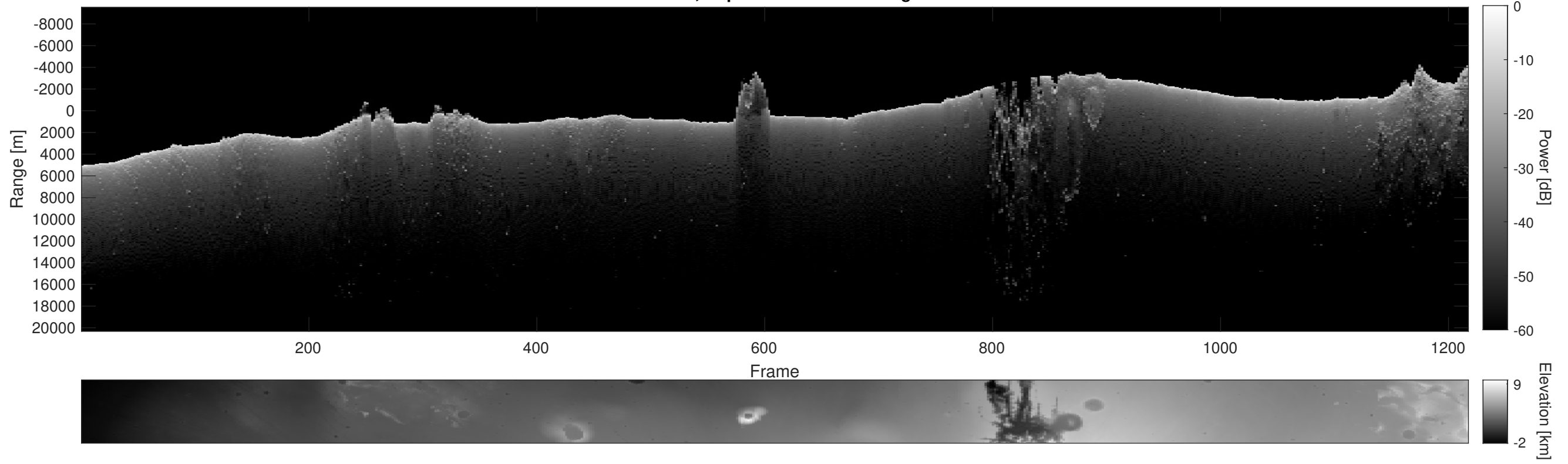
Orbit 11425, Depth-Corrected Cluttergram
