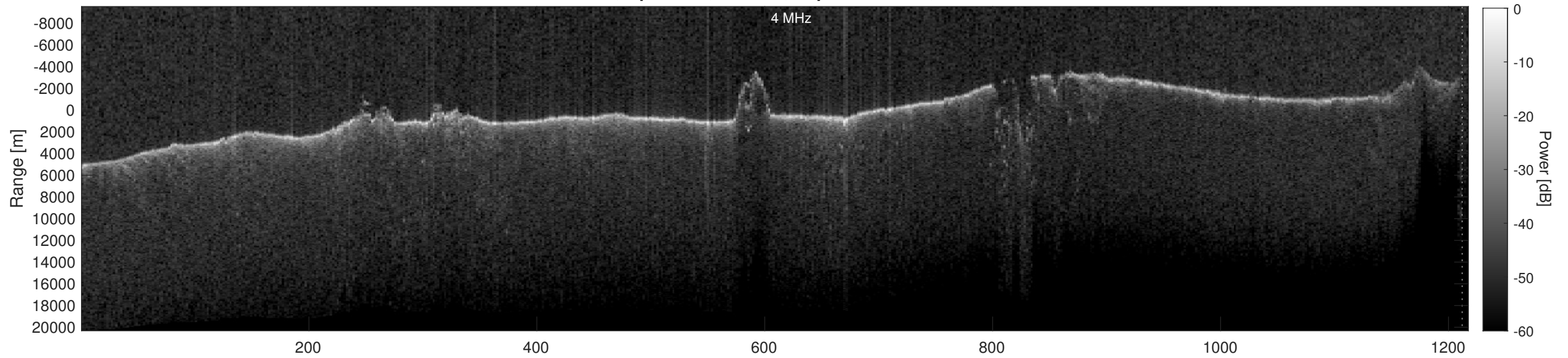
Orbit 11425, Depth-Corrected Cluttergram
