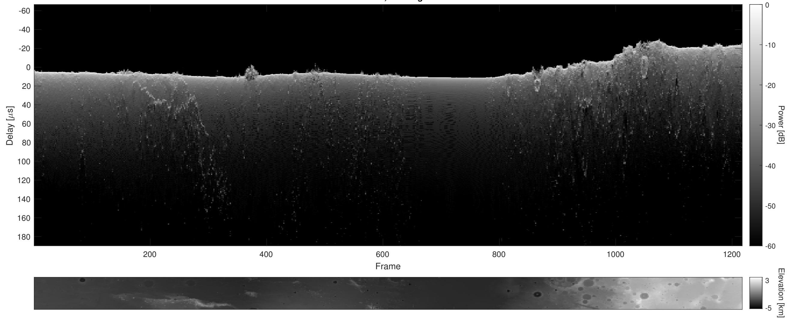
Orbit 11426, Cluttergram
