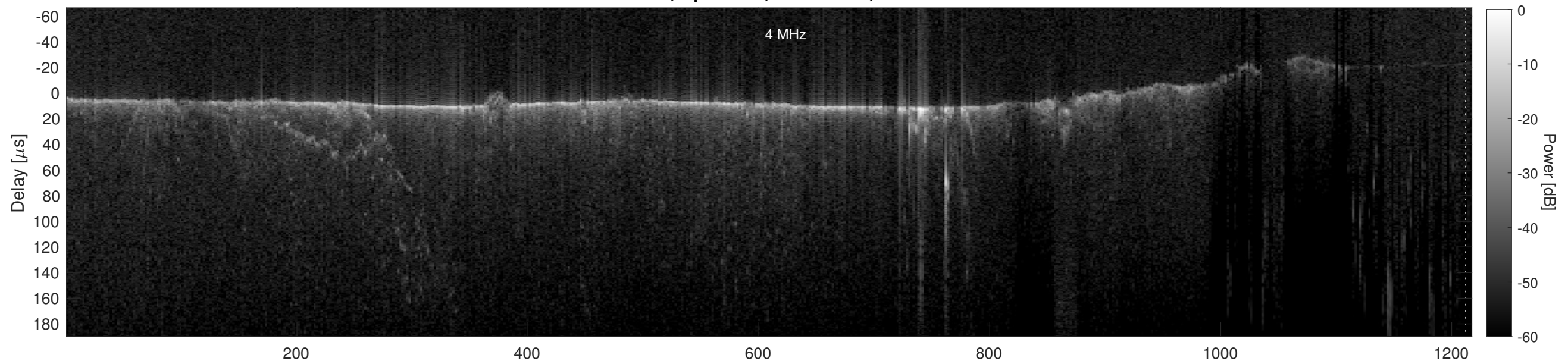
Orbit 11426, Cluttergram
