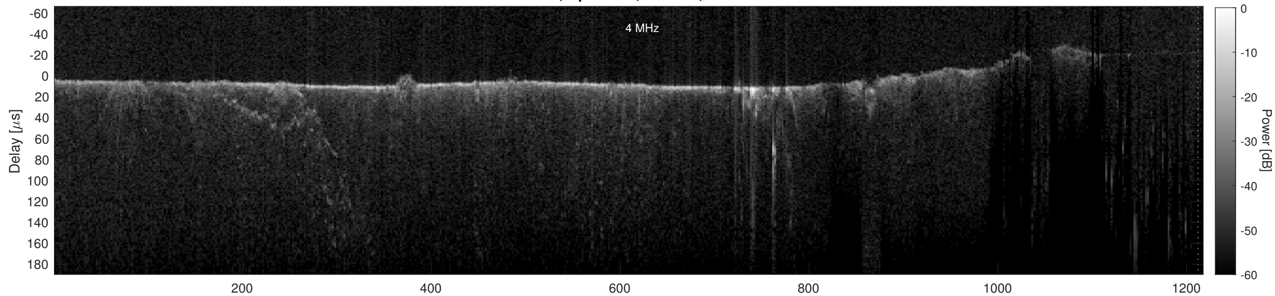
Orbit 11426, Cluttergram
