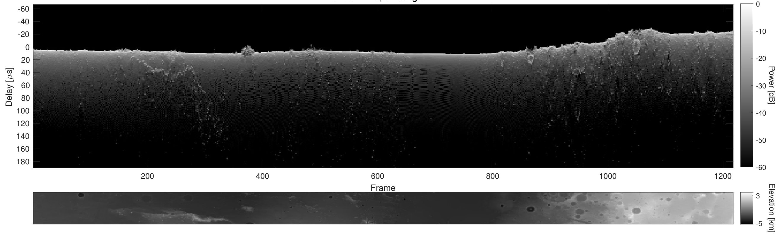
Orbit 11426, Cluttergram
