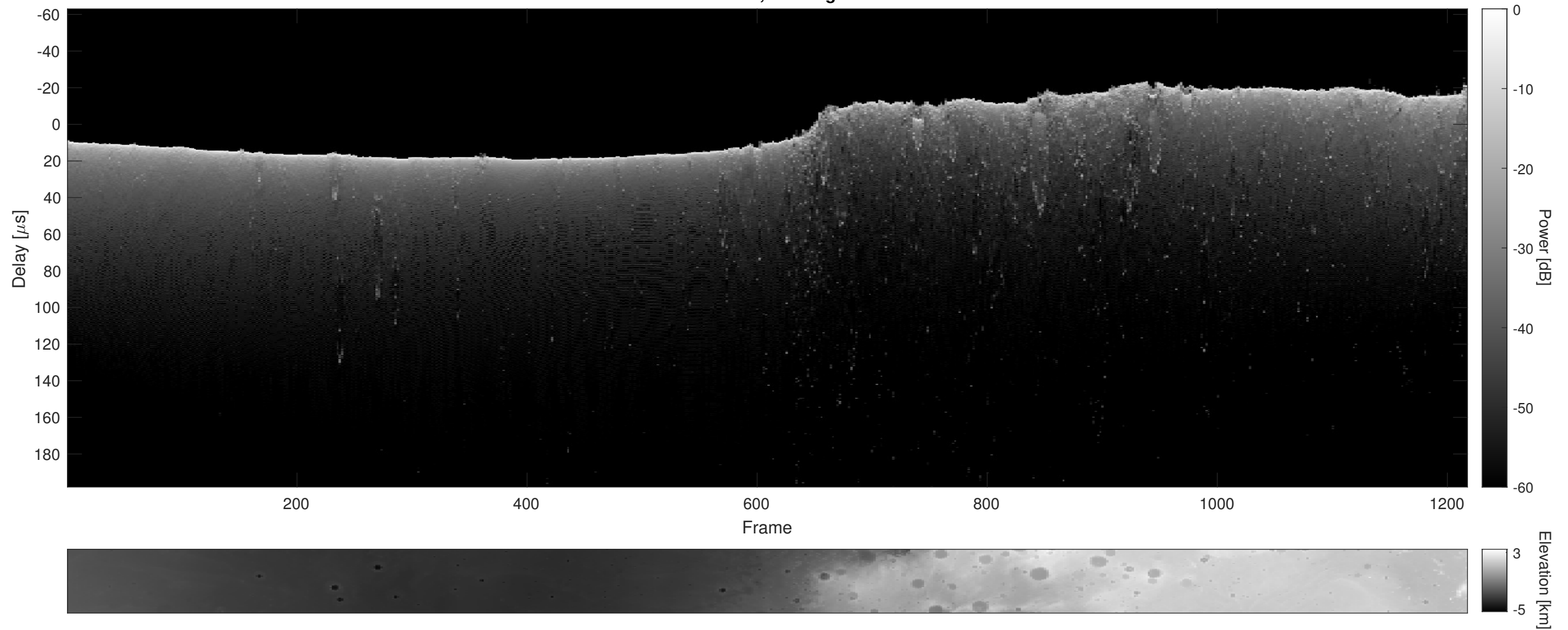
Orbit 11430, Cluttergram
