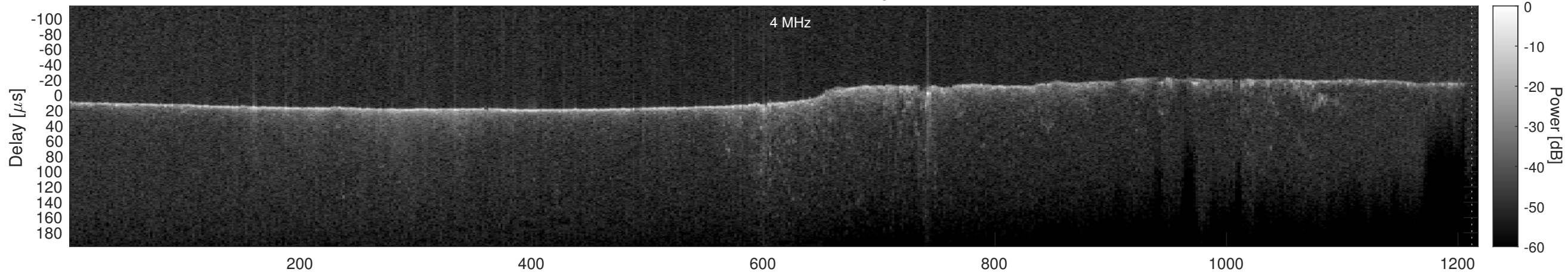
Orbit 11430, Cluttergram
