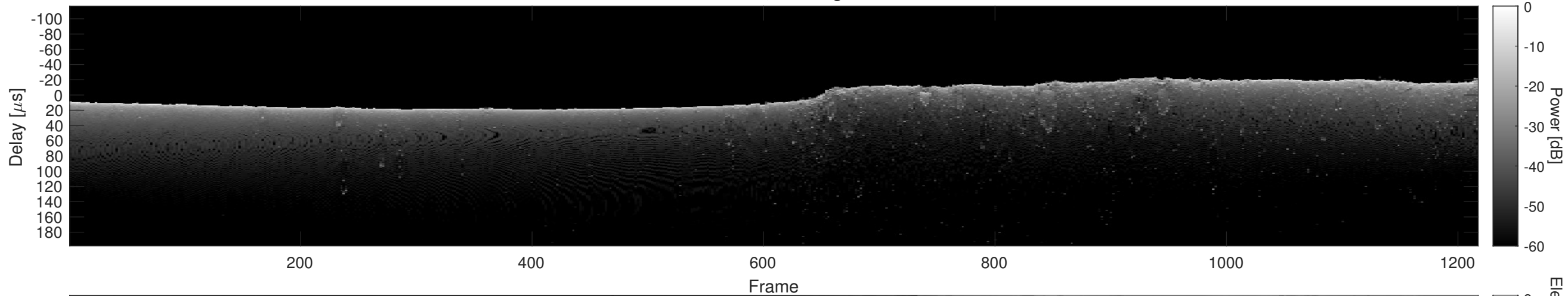
Orbit 11430, Cluttergram
