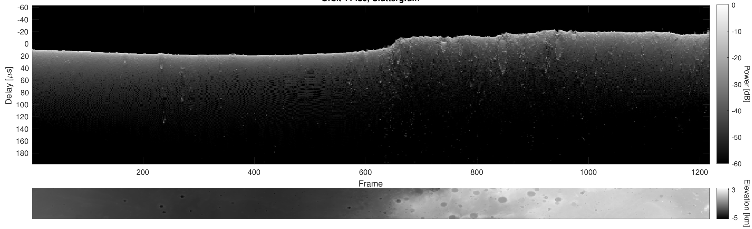
Orbit 11430, Cluttergram
