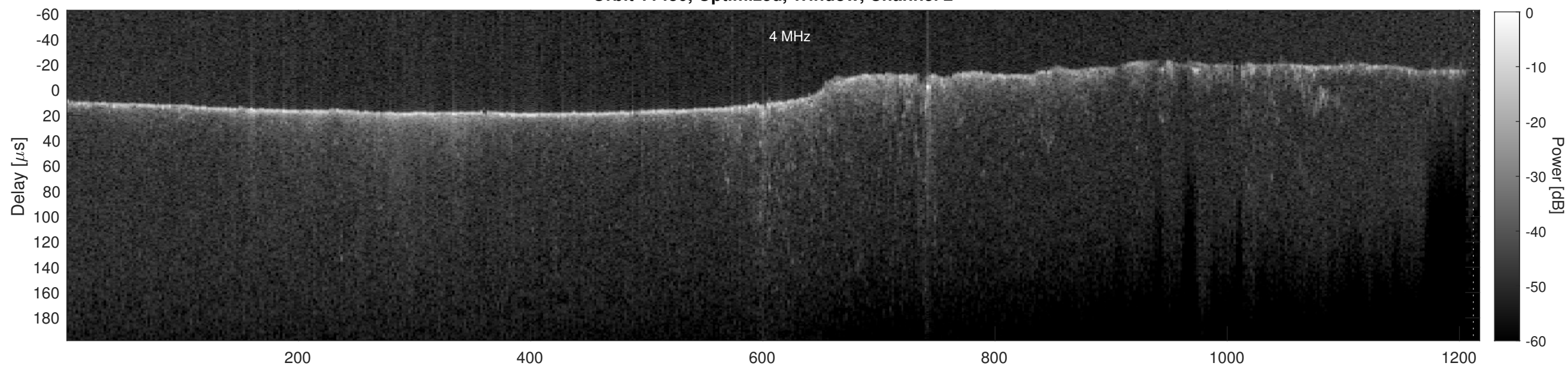
Orbit 11430, Cluttergram
