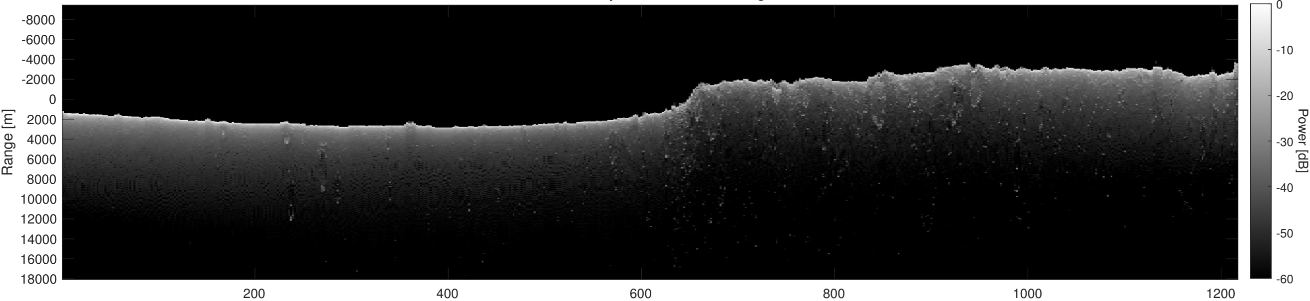
Orbit 11430, Depth-Corrected Cluttergram
