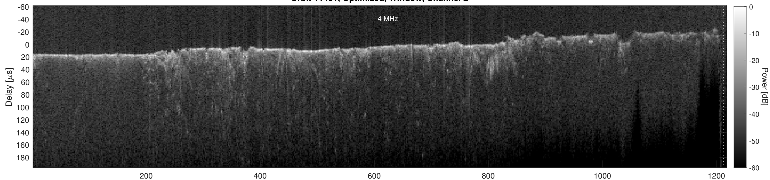
Orbit 11431, Cluttergram
