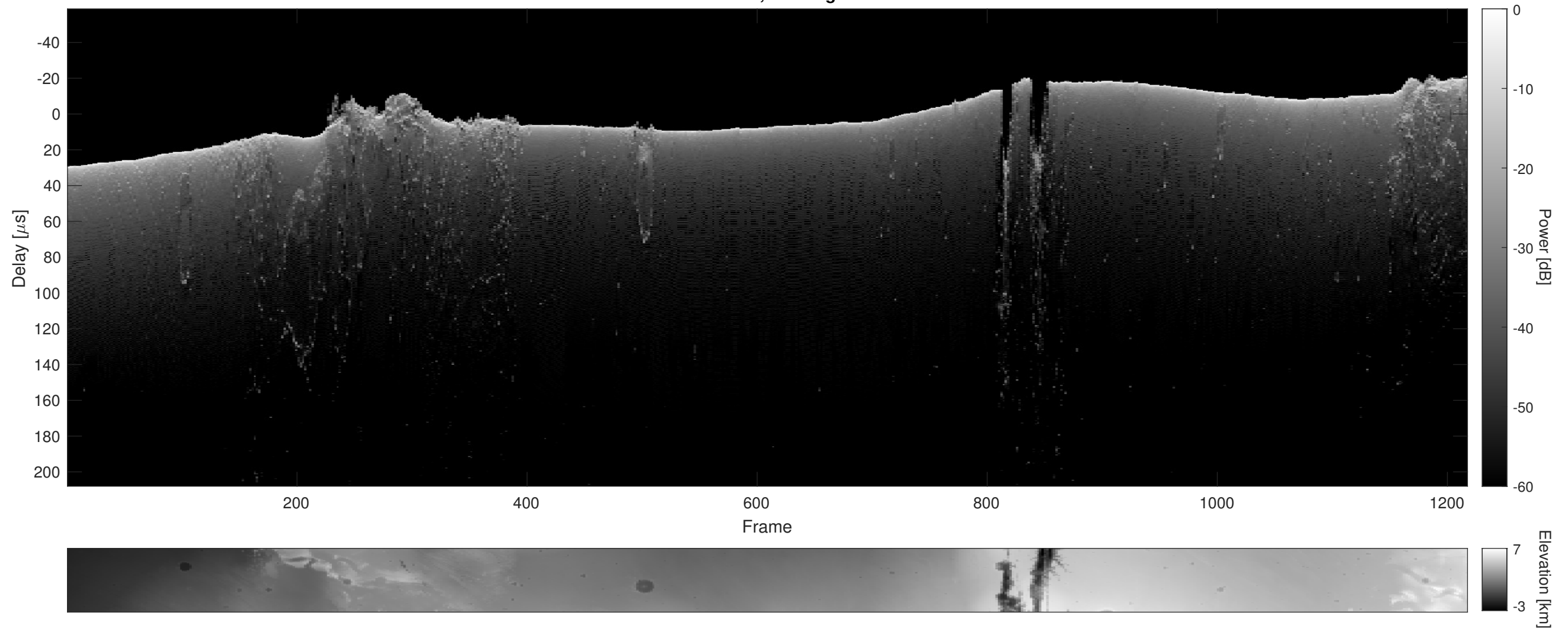
Orbit 11432, Cluttergram
